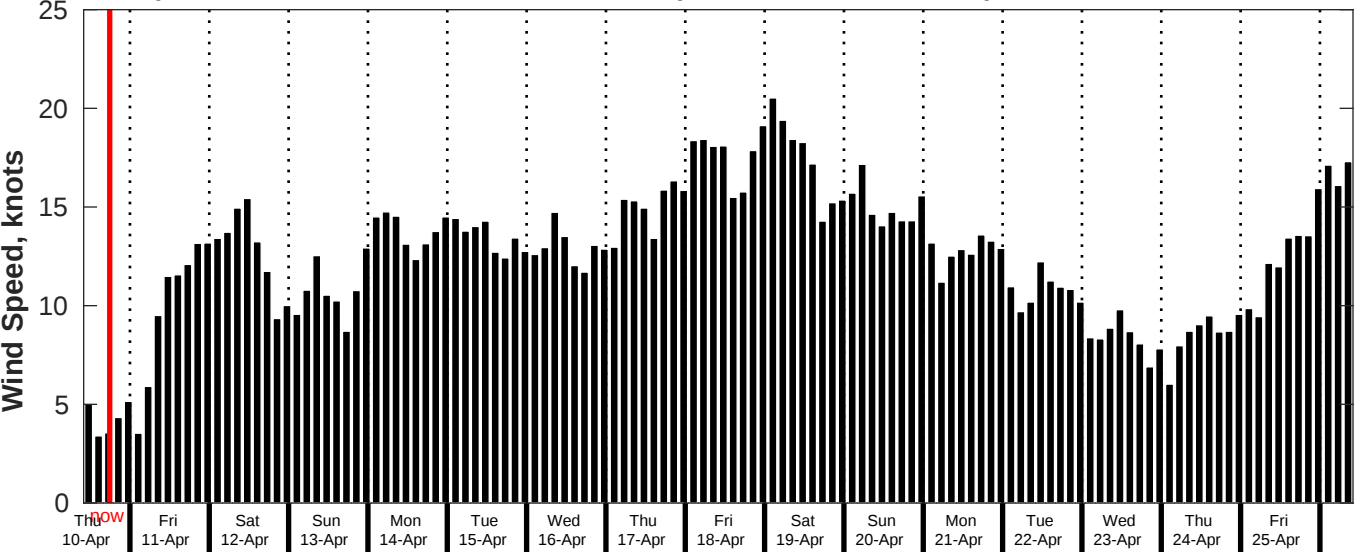
GFS Wind Speed Forecast for NDBC 52211 from 09-Apr-2025 10:00:00 to 25-Apr-2025 10:00:00
