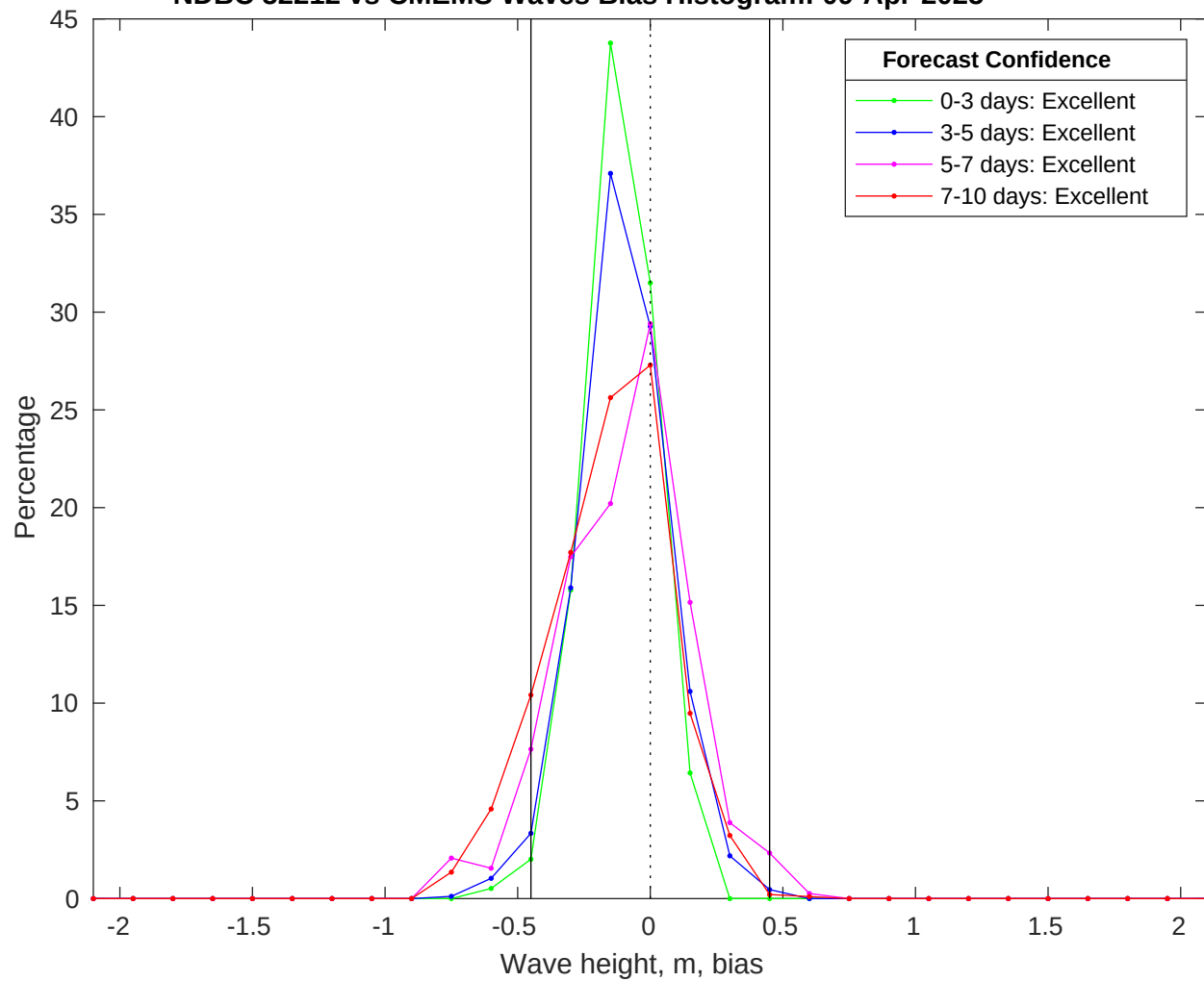
NDBC 52212 vs CMEMS Waves Bias Histogram: 09-Apr-2025
