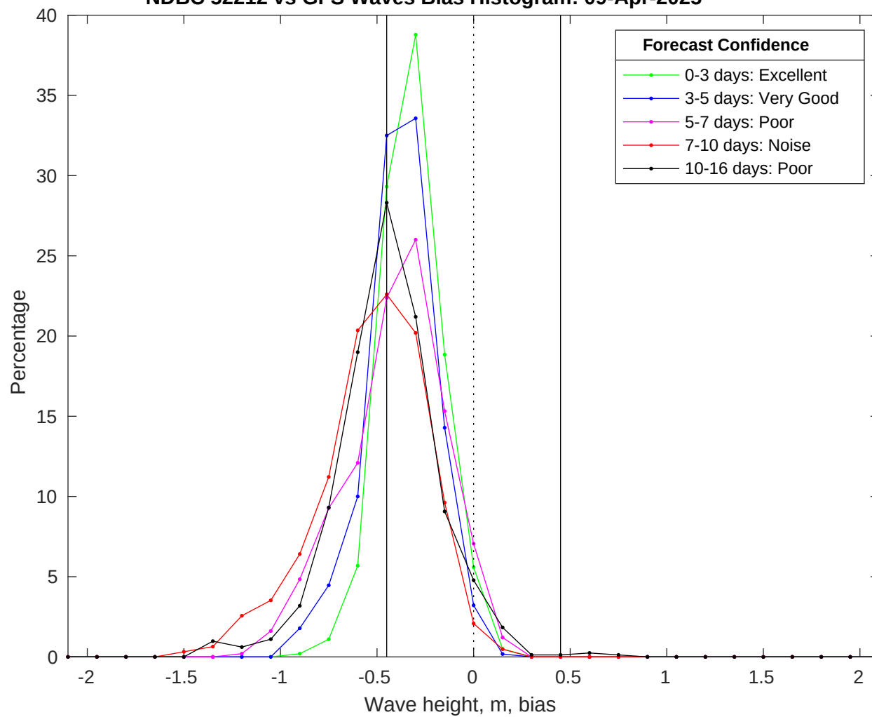
NDBC 52212 vs GFS Waves Bias Histogram: 09-Apr-2025
