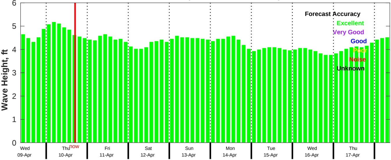
CMEMS Wave Forecast for NDBC 52212 from 08-Apr-2025 09:00:00 to 17-Apr-2025 09:00:00
