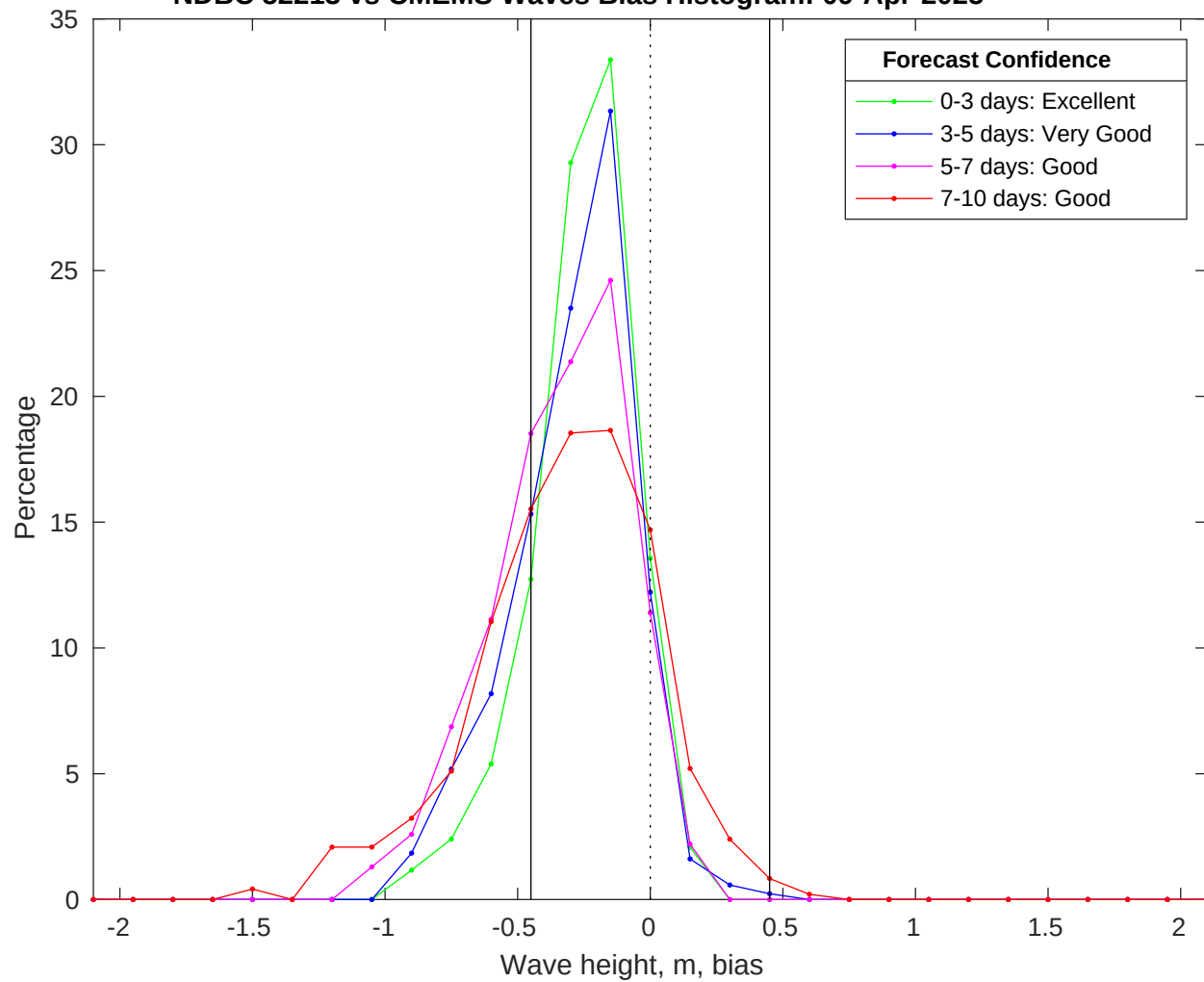
NDBC 52213 vs CMEMS Waves Bias Histogram: 09-Apr-2025
