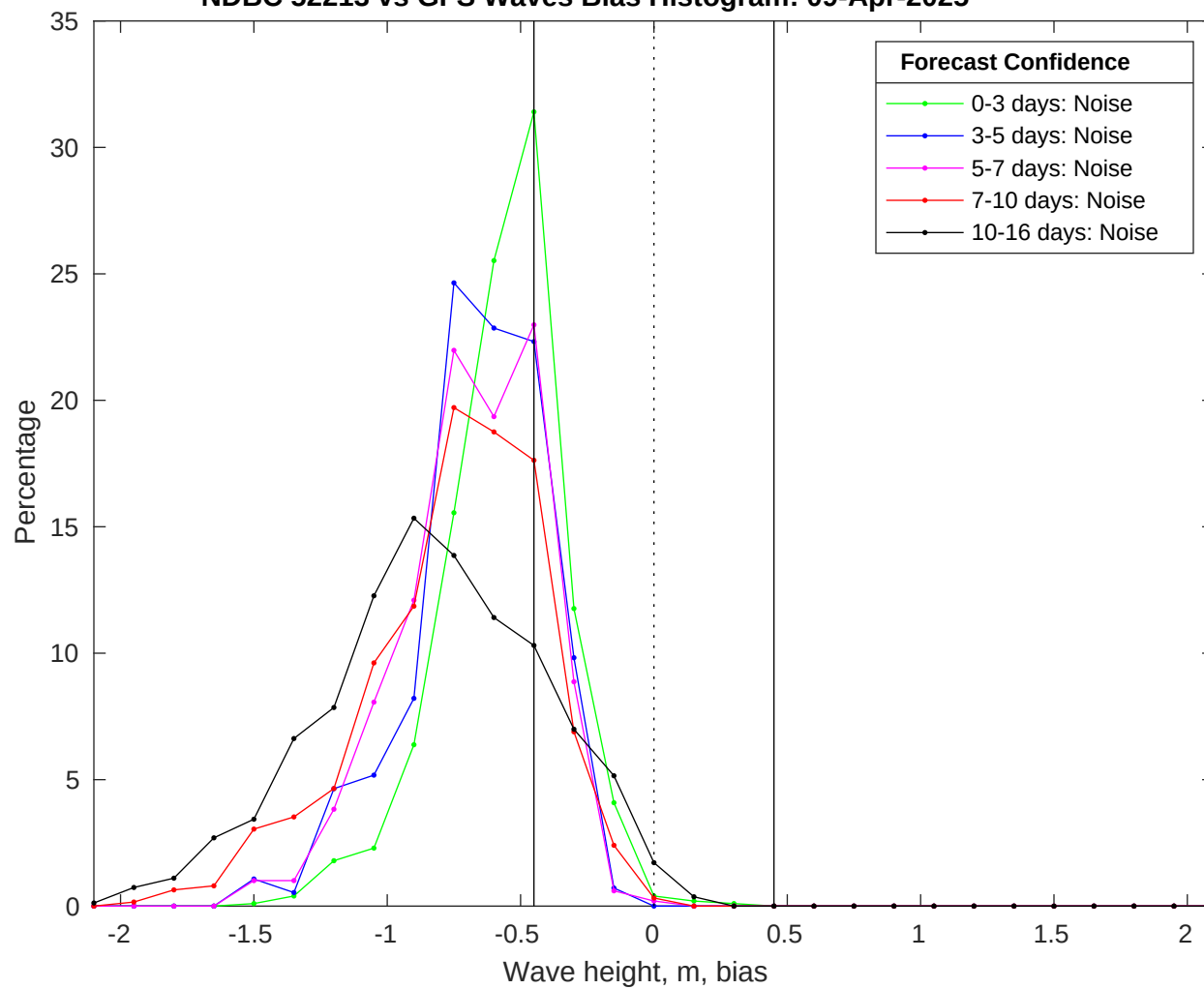
NDBC 52213 vs GFS Waves Bias Histogram: 09-Apr-2025
