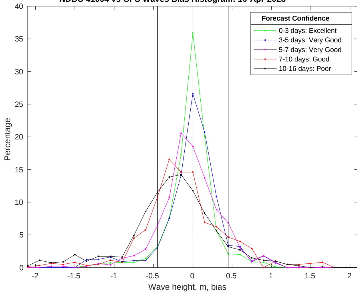
NDBC 41004 vs GFS Waves Bias Histogram: 10-Apr-2025
