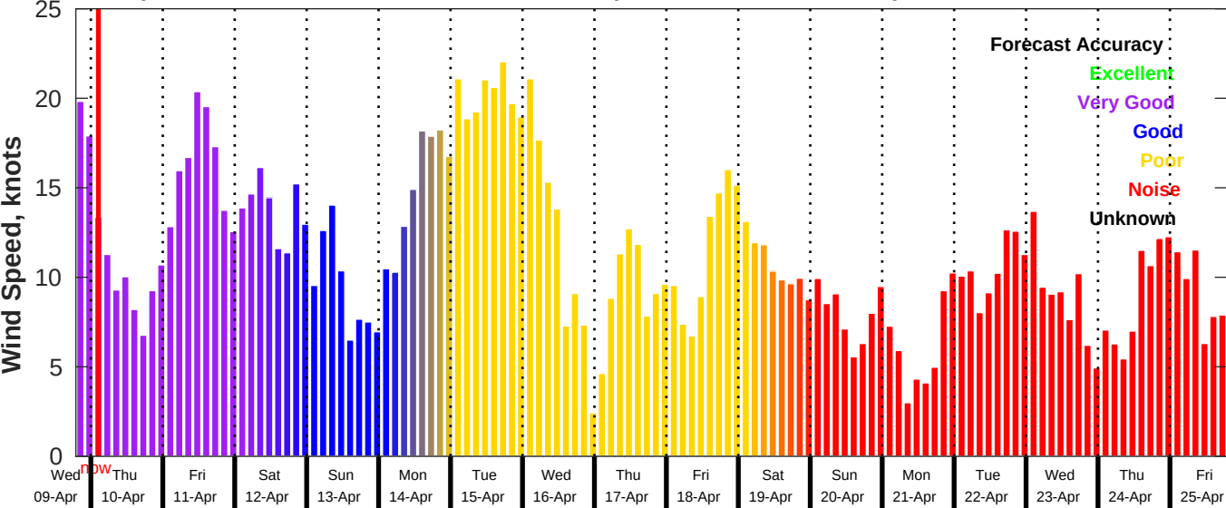
GFS Wind Speed Forecast for NDBC 41004 from 09-Apr-2025 19:00:00 to 25-Apr-2025 19:00:00
