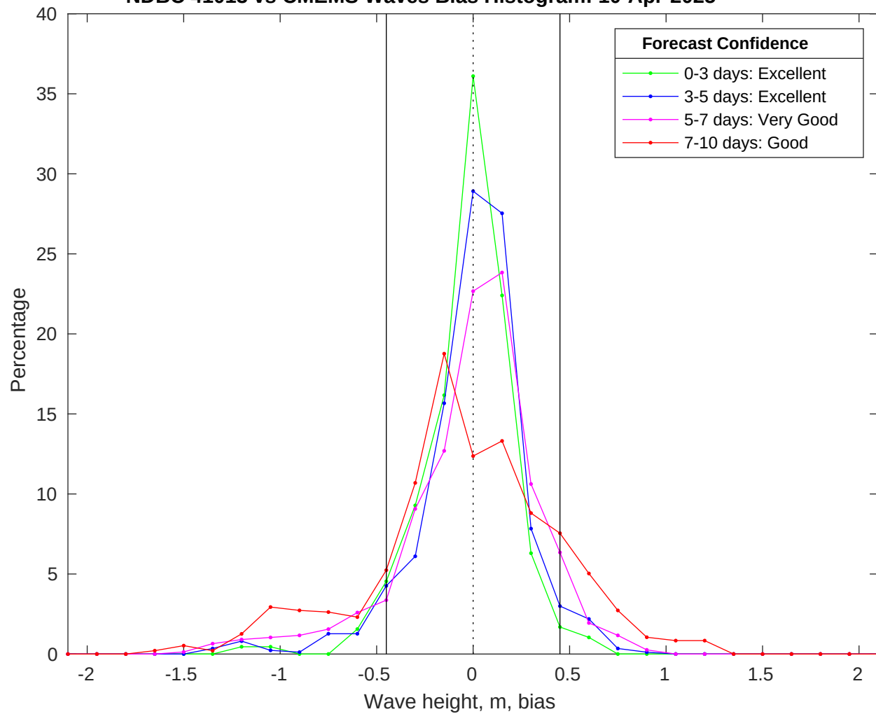
NDBC 41013 vs CMEMS Waves Bias Histogram: 10-Apr-2025
