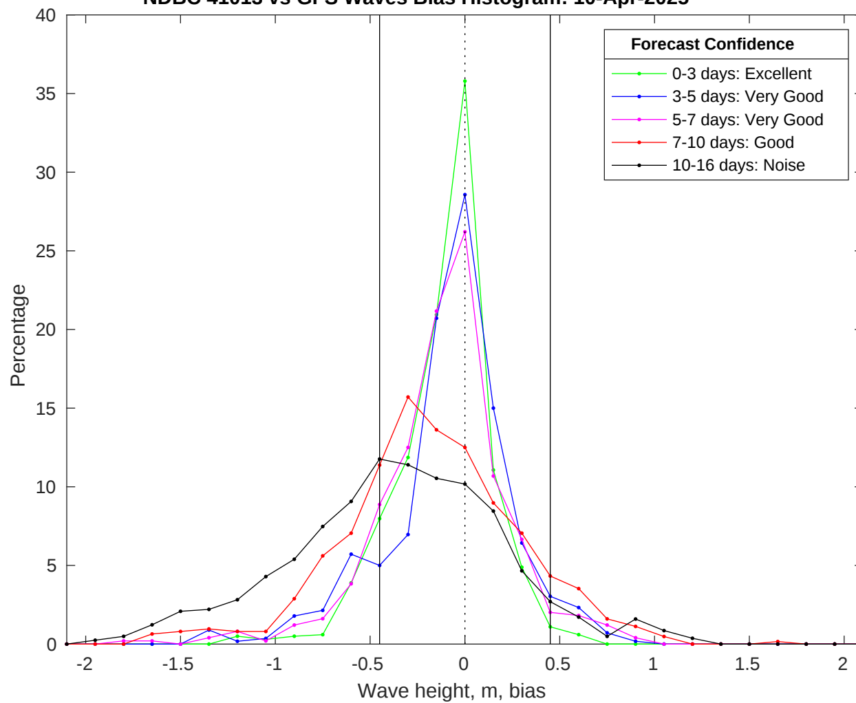
NDBC 41013 vs GFS Waves Bias Histogram: 10-Apr-2025
