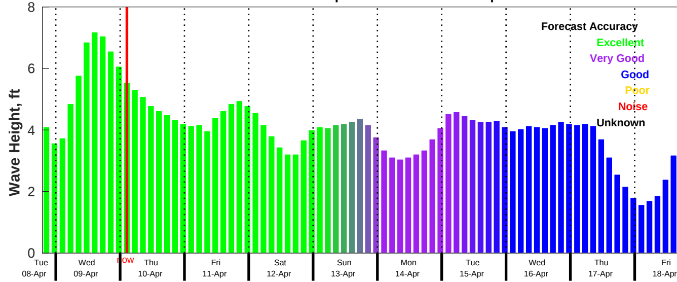
CMEMS Wave Forecast for NDBC 41013 from 08-Apr-2025 19:00:00 to 18-Apr-2025 19:00:00
