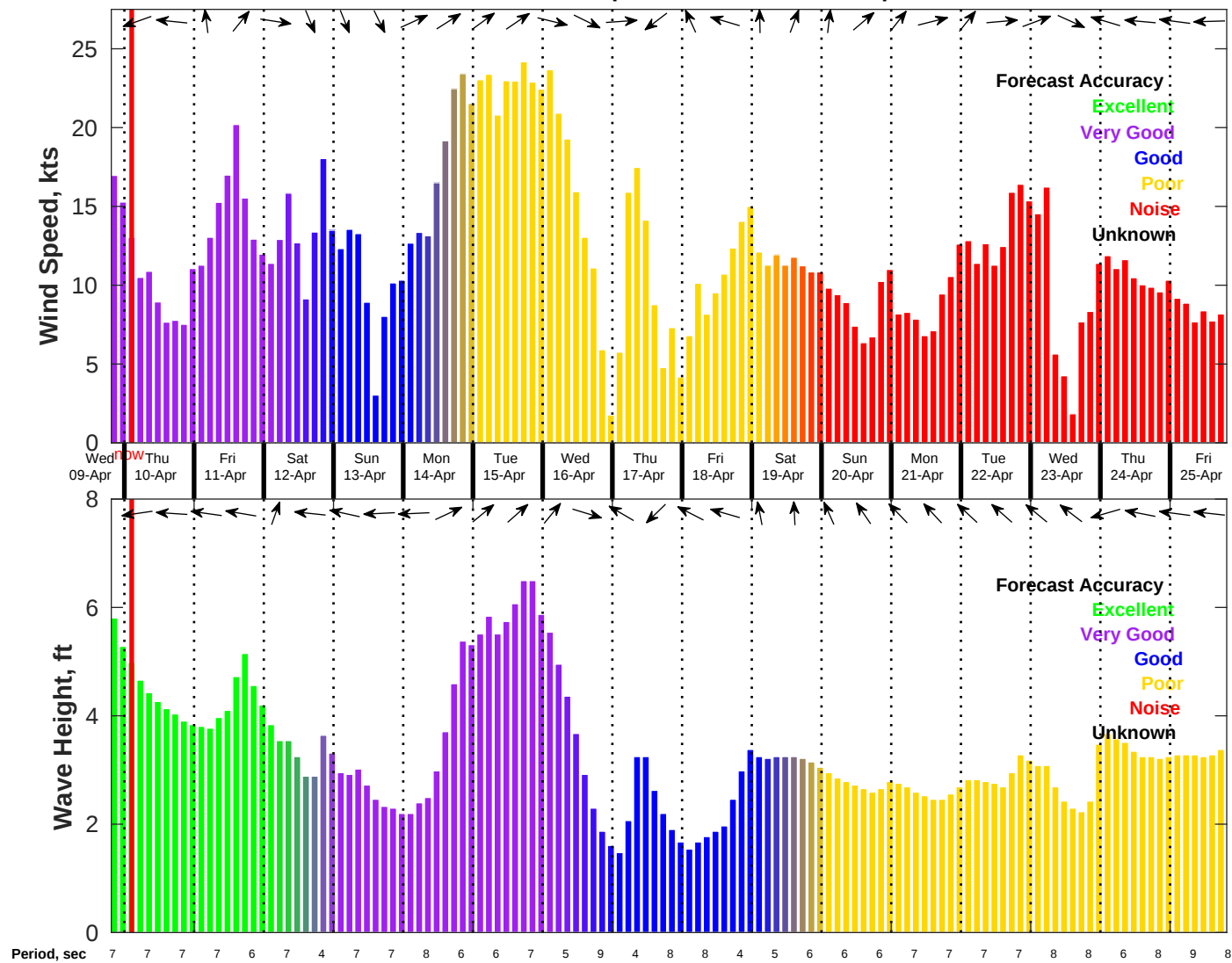
Wind & Wave Forecast for NDBC 41013 from 09-Apr-2025 19:00:00 to 25-Apr-2025 19:00:00
