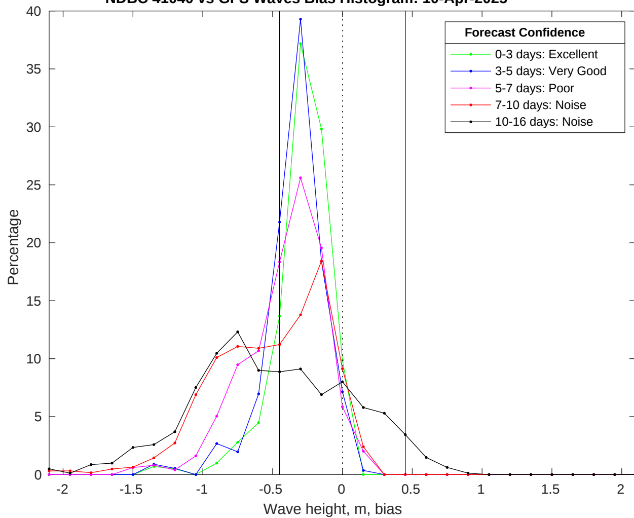
NDBC 41040 vs GFS Waves Bias Histogram: 10-Apr-2025
