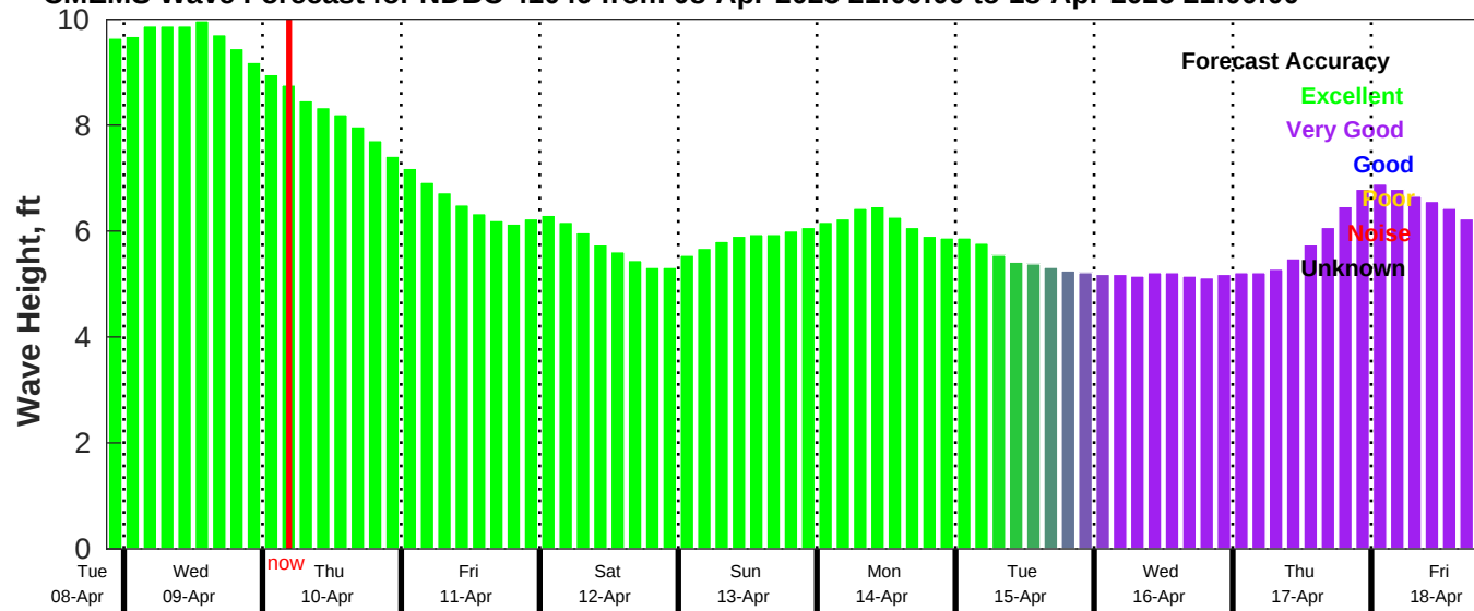
CMEMS Wave Forecast for NDBC 41040 from 08-Apr-2025 21:00:00 to 18-Apr-2025 21:00:00
