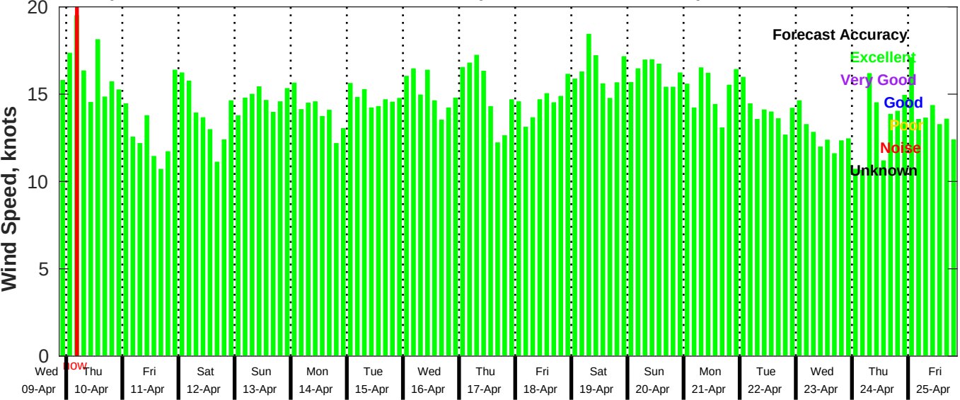
GFS Wind Speed Forecast for NDBC 41040 from 09-Apr-2025 21:00:00 to 25-Apr-2025 21:00:00
