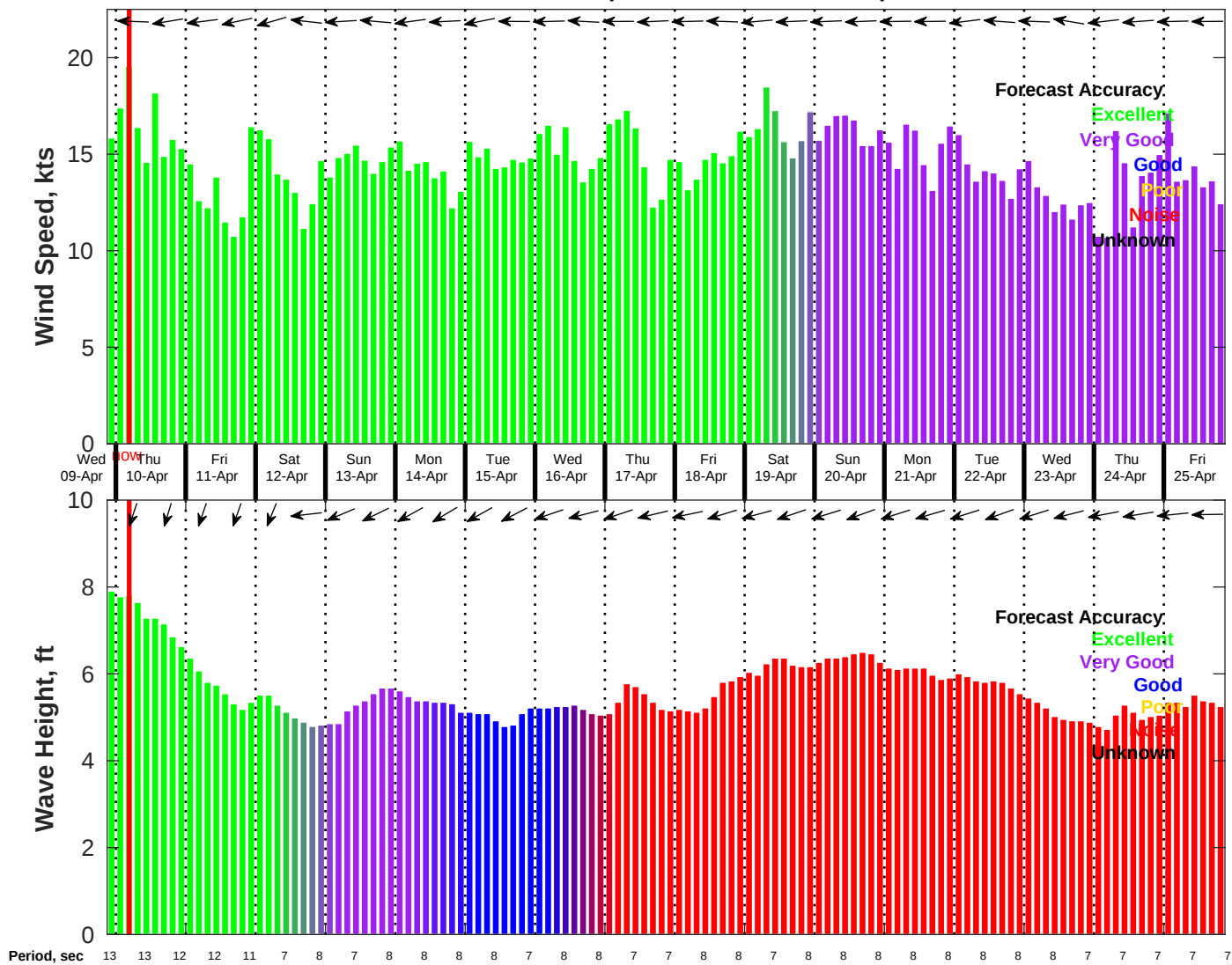
Wind & Wave Forecast for NDBC 41040 from 09-Apr-2025 21:00:00 to 25-Apr-2025 21:00:00
