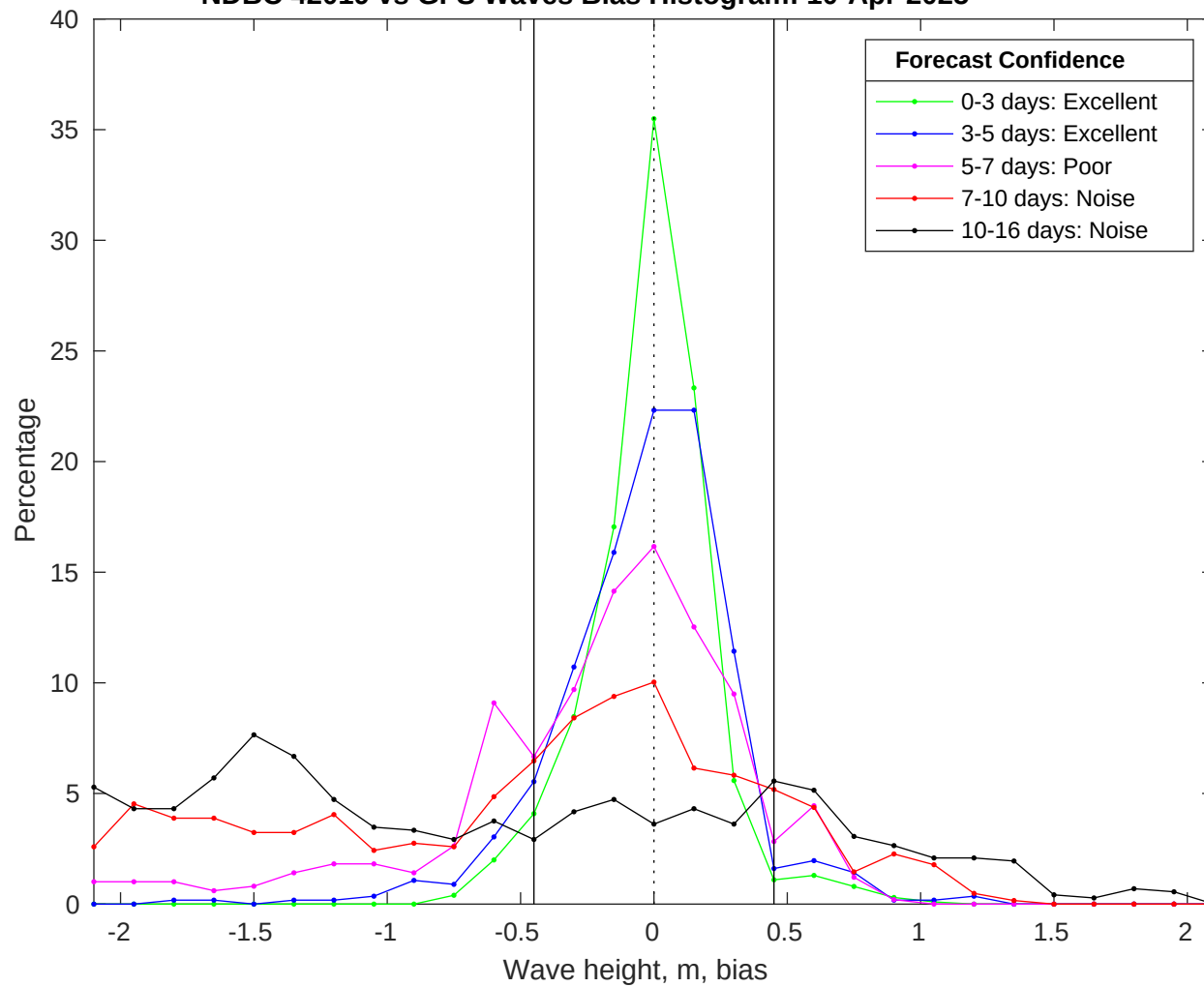
NDBC 42019 vs GFS Waves Bias Histogram: 10-Apr-2025
