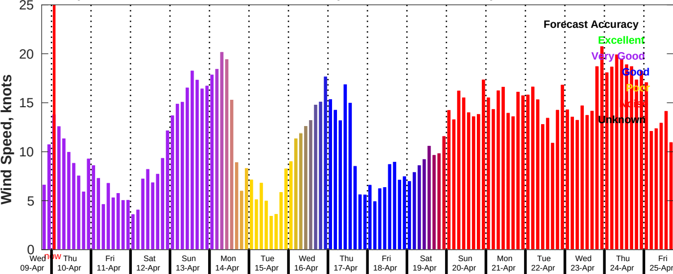
GFS Wind Speed Forecast for NDBC 42019 from 09-Apr-2025 18:00:00 to 25-Apr-2025 18:00:00
