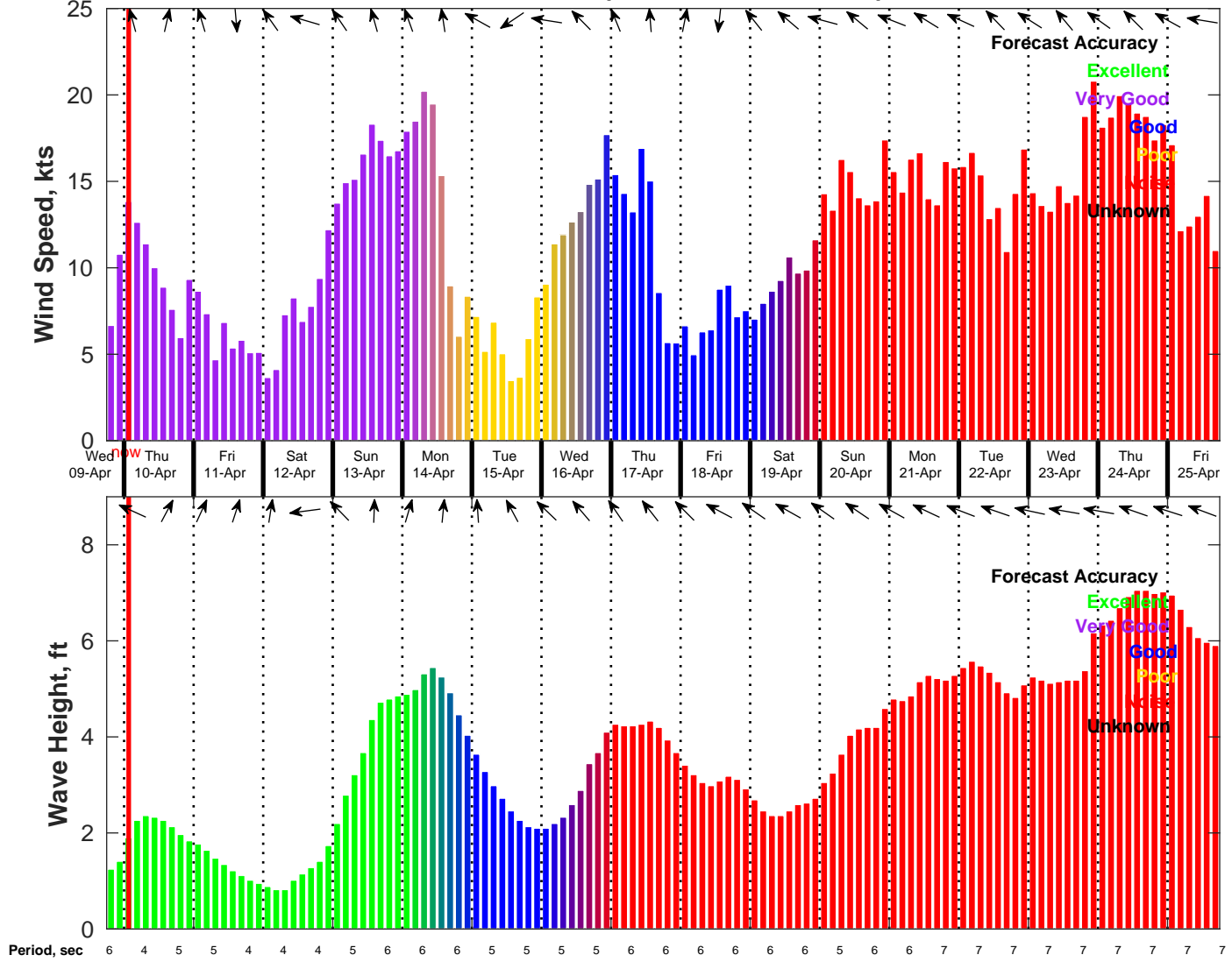
Wind & Wave Forecast for NDBC 42019 from 09-Apr-2025 18:00:00 to 25-Apr-2025 18:00:00
