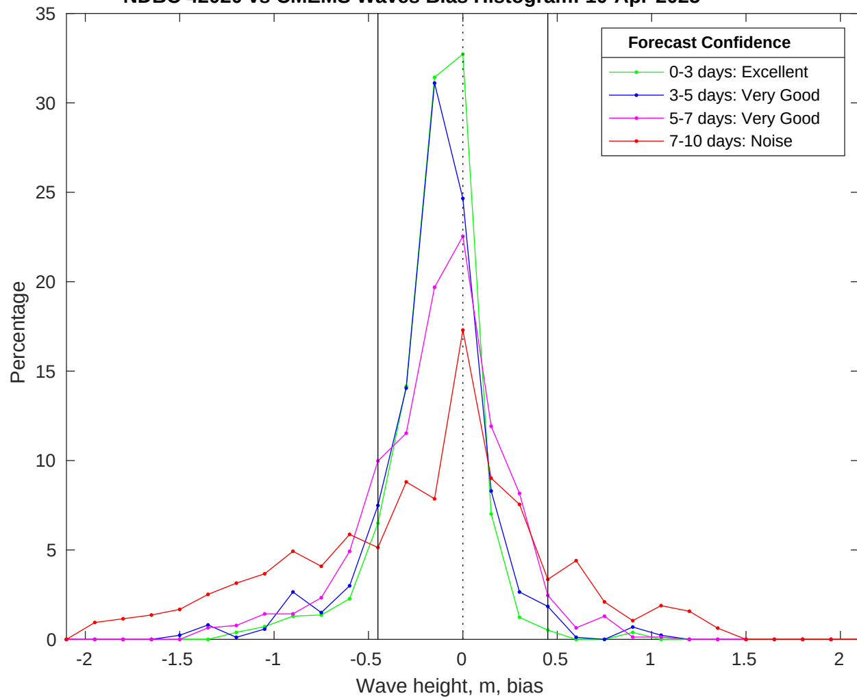
NDBC 42020 vs CMEMS Waves Bias Histogram: 10-Apr-2025
