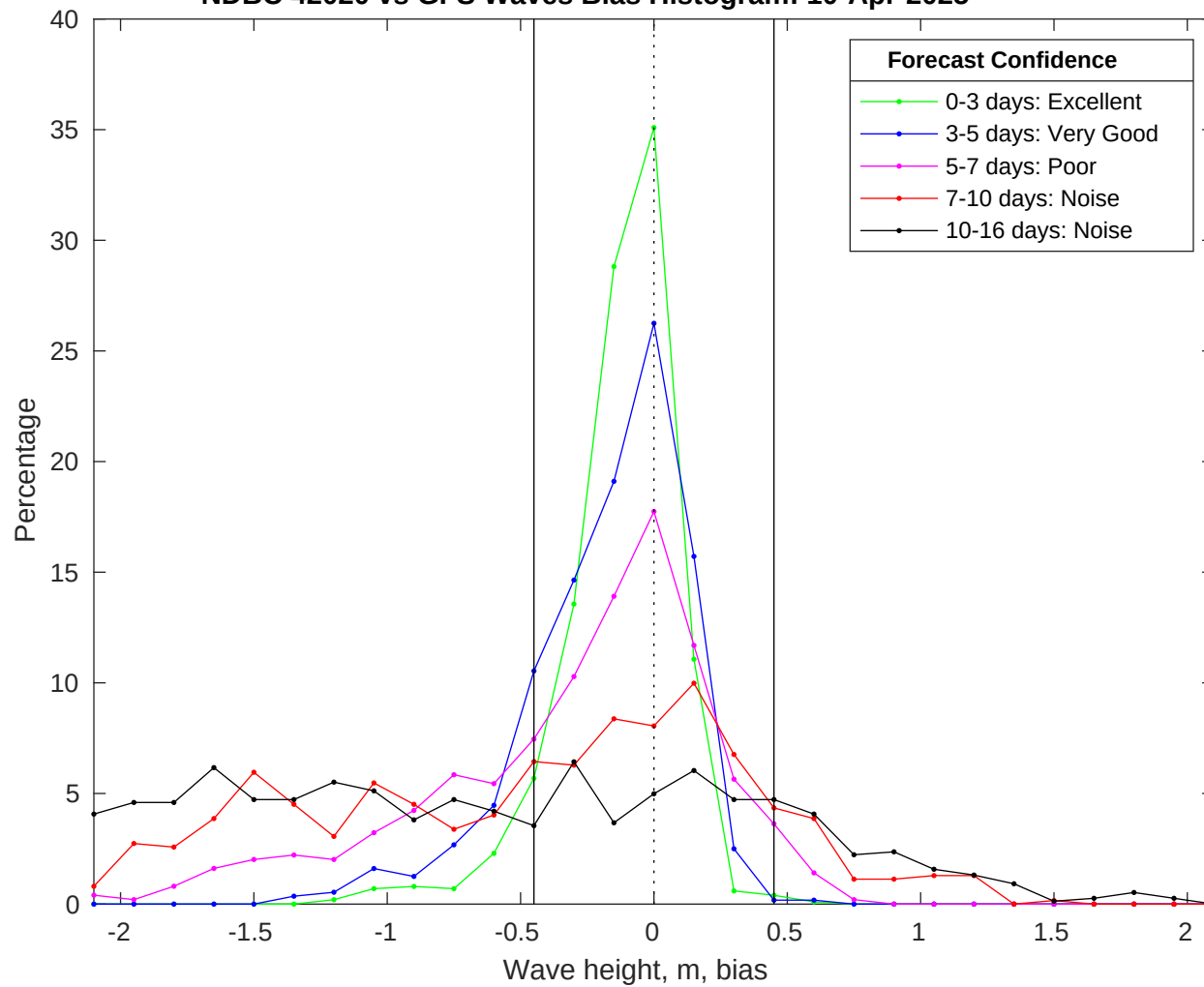
NDBC 42020 vs GFS Waves Bias Histogram: 10-Apr-2025
