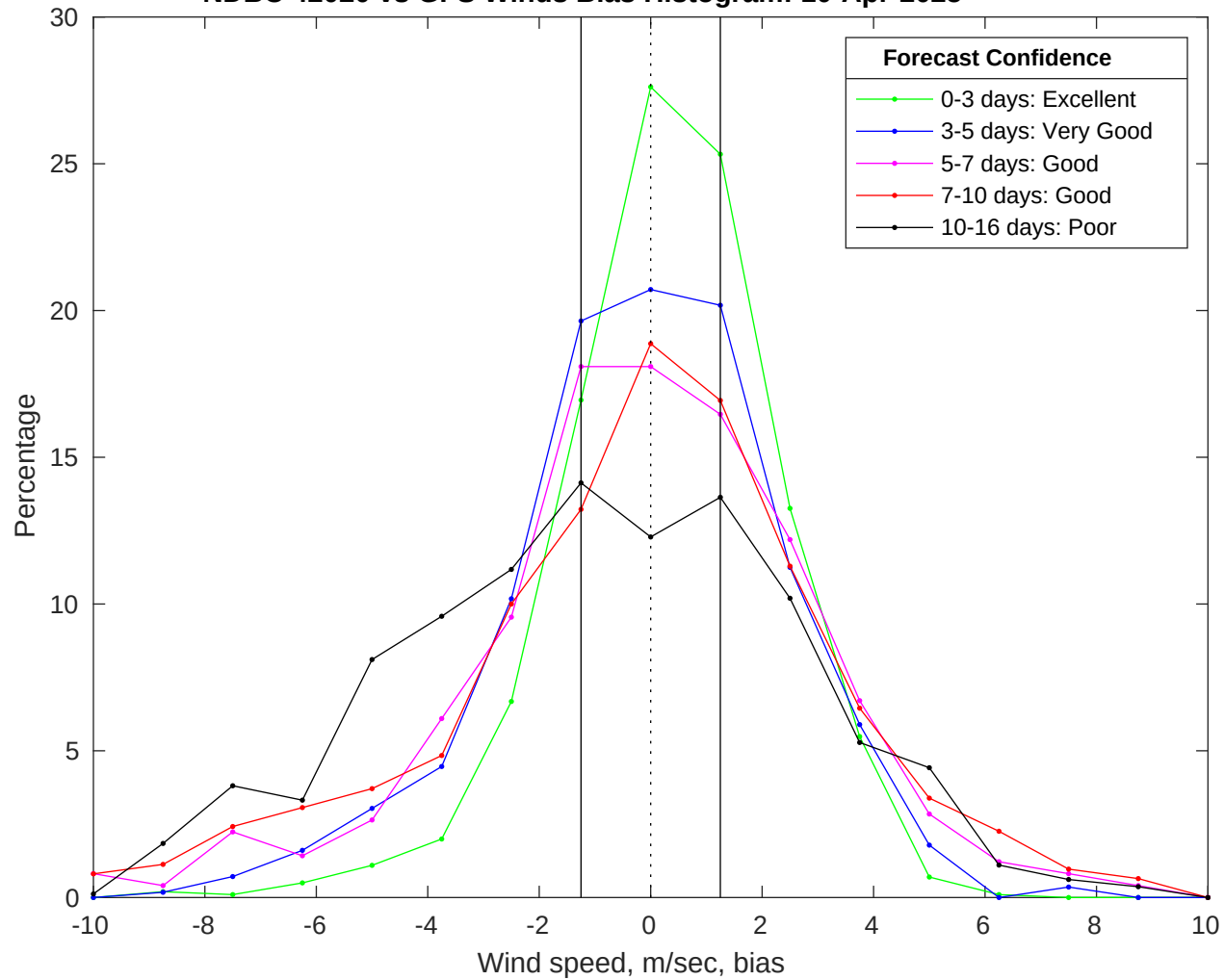
NDBC 42020 vs GFS Winds Bias Histogram: 10-Apr-2025
