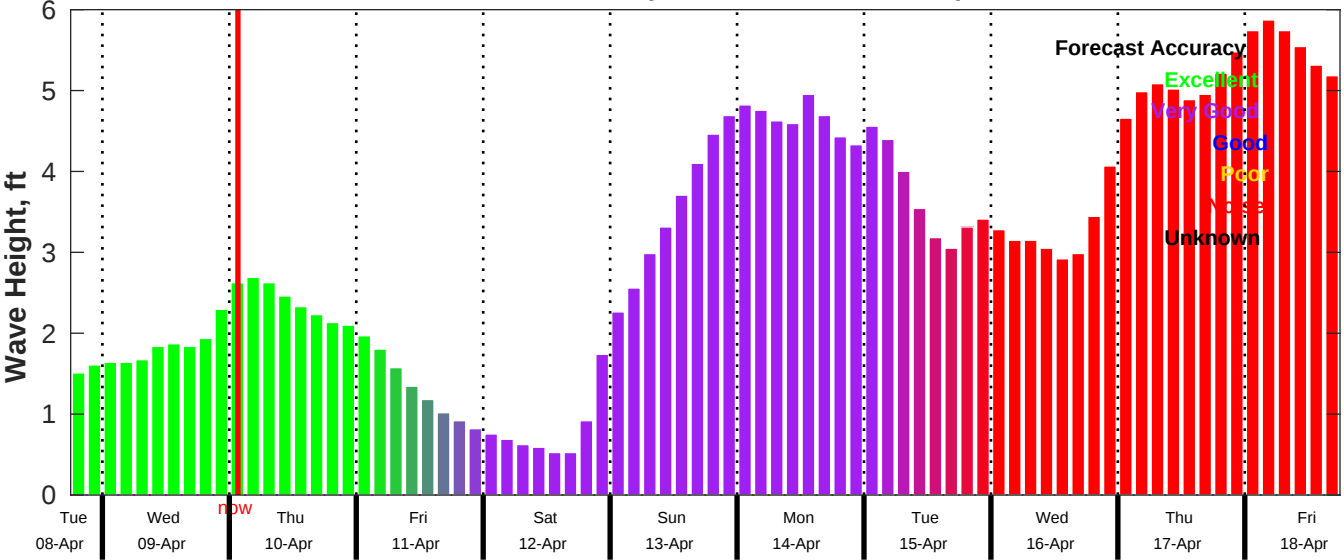
CMEMS Wave Forecast for NDBC 42020 from 08-Apr-2025 18:00:00 to 18-Apr-2025 18:00:00
