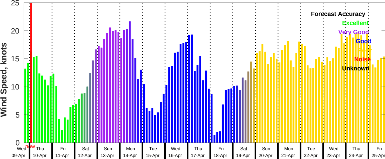
GFS Wind Speed Forecast for NDBC 42020 from 09-Apr-2025 18:00:00 to 25-Apr-2025 18:00:00
