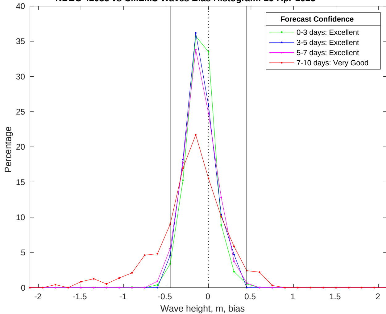
NDBC 42035 vs CMEMS Waves Bias Histogram: 10-Apr-2025
