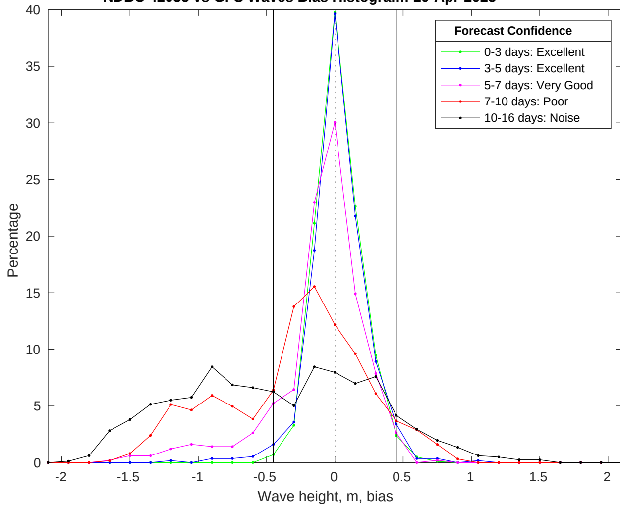
NDBC 42035 vs GFS Waves Bias Histogram: 10-Apr-2025
