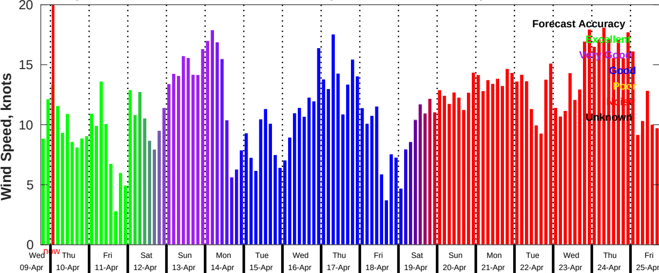
GFS Wind Speed Forecast for NDBC 42035 from 09-Apr-2025 18:00:00 to 25-Apr-2025 18:00:00
