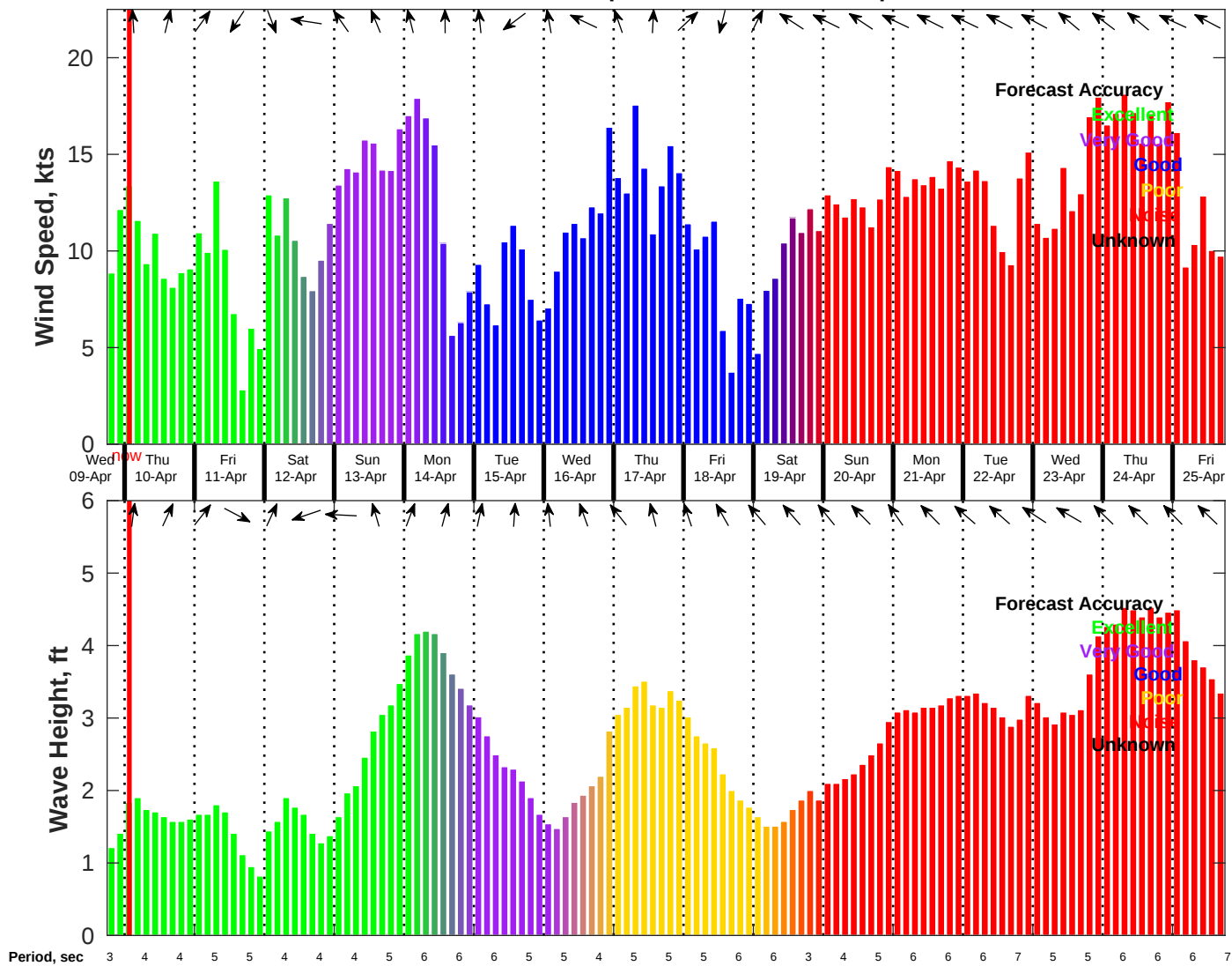
Wind & Wave Forecast for NDBC 42035 from 09-Apr-2025 18:00:00 to 25-Apr-2025 18:00:00
