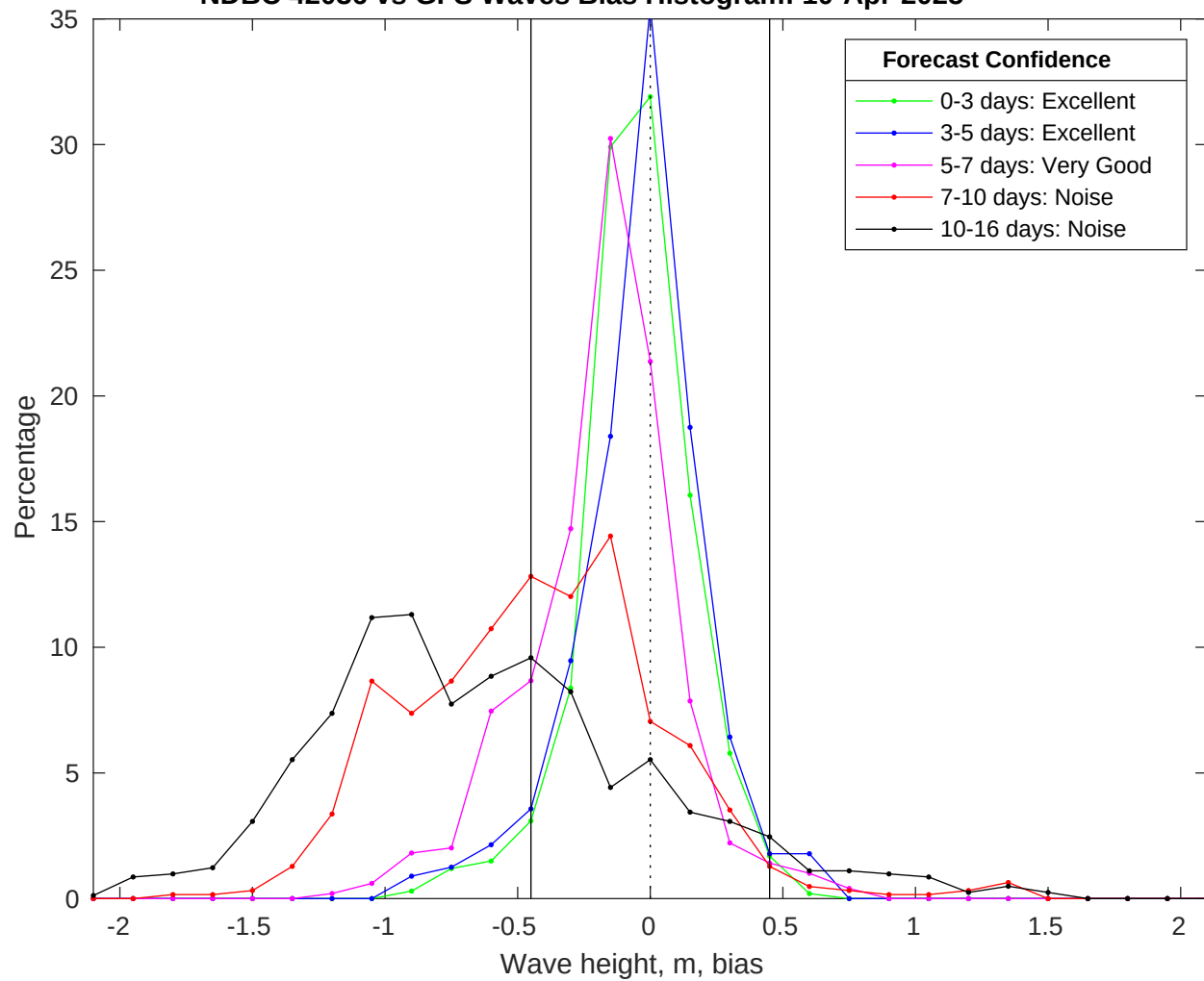
NDBC 42036 vs GFS Waves Bias Histogram: 10-Apr-2025
