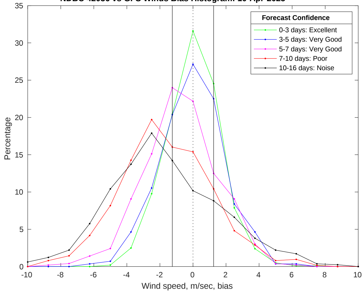
NDBC 42036 vs GFS Winds Bias Histogram: 10-Apr-2025
