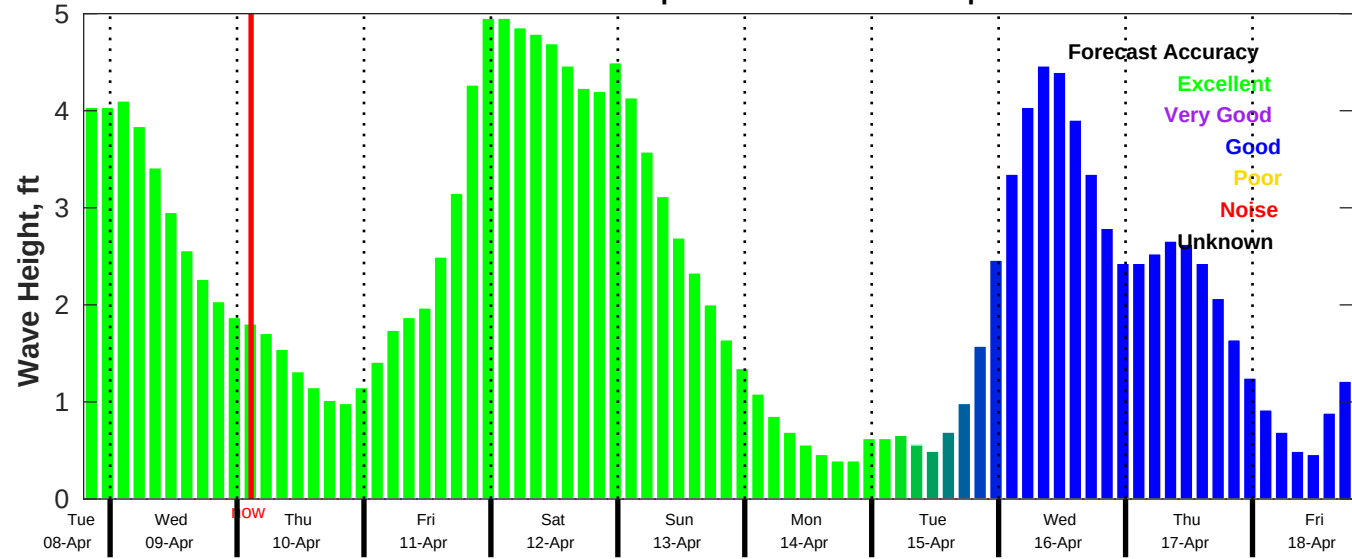
CMEMS Wave Forecast for NDBC 42036 from 08-Apr-2025 19:00:00 to 18-Apr-2025 19:00:00
