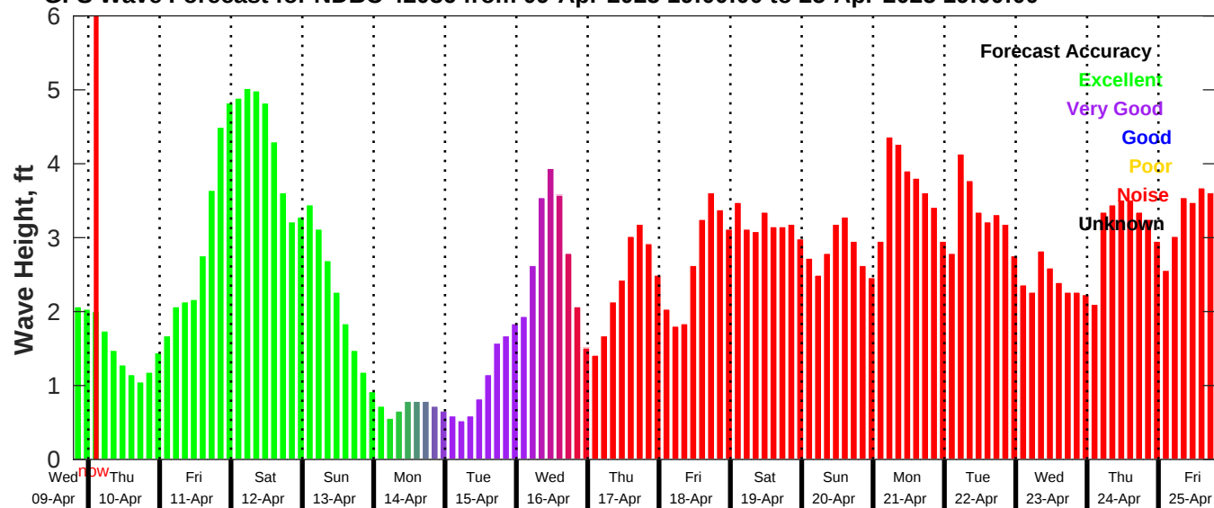
GFS Wave Forecast for NDBC 42036 from 09-Apr-2025 19:00:00 to 25-Apr-2025 19:00:00
