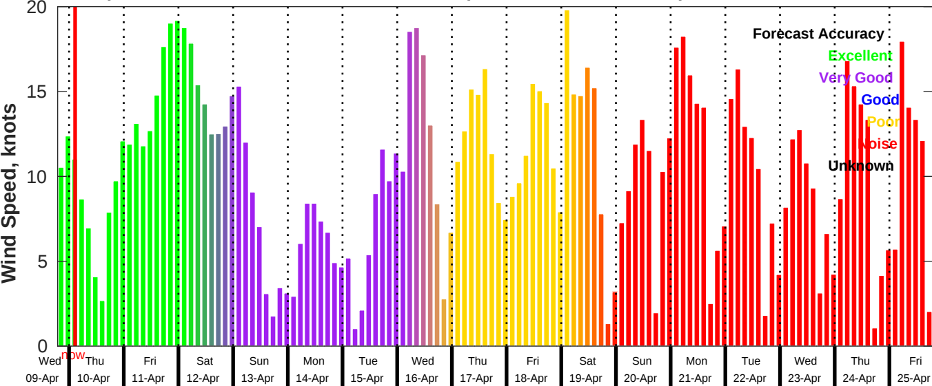
GFS Wind Speed Forecast for NDBC 42036 from 09-Apr-2025 19:00:00 to 25-Apr-2025 19:00:00
