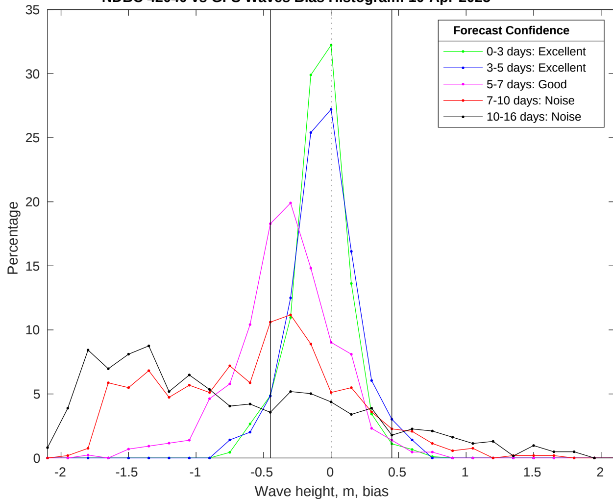
NDBC 42040 vs GFS Waves Bias Histogram: 10-Apr-2025
