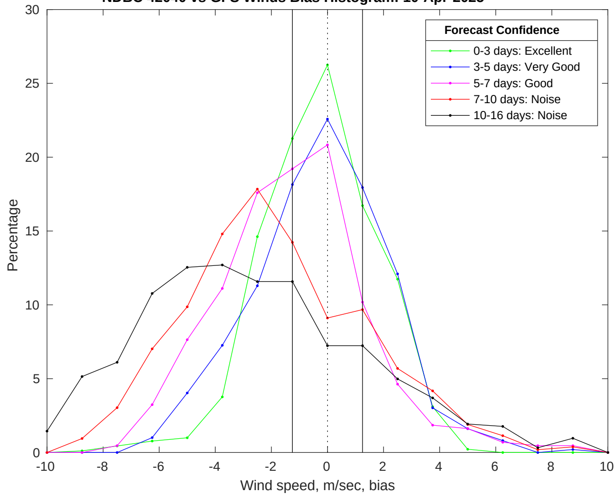
NDBC 42040 vs GFS Winds Bias Histogram: 10-Apr-2025
