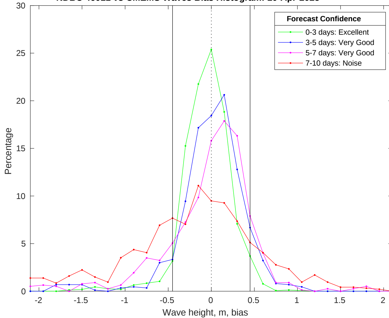
NDBC 46011 vs CMEMS Waves Bias Histogram: 10-Apr-2025
