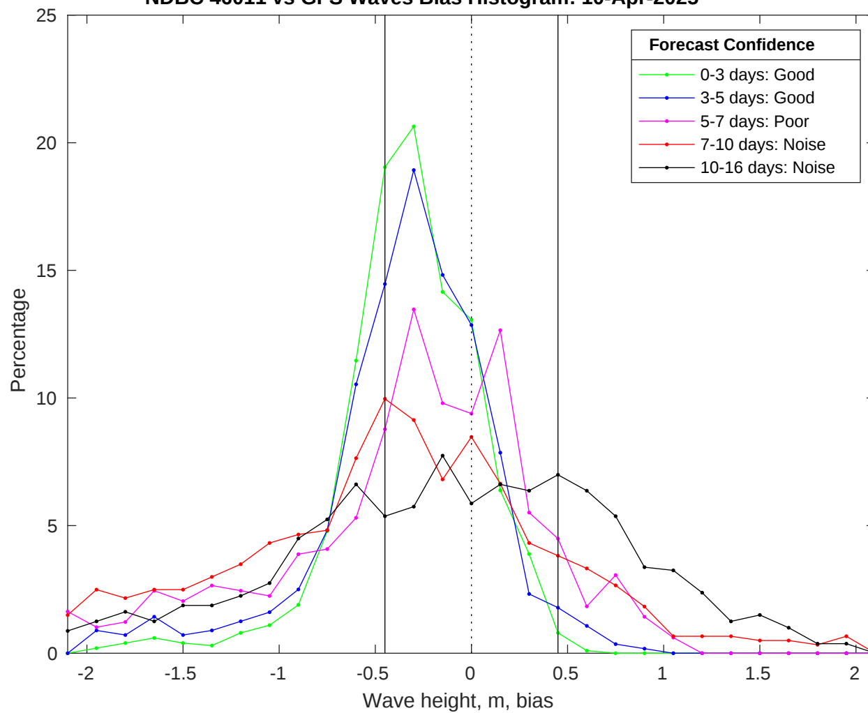
NDBC 46011 vs GFS Waves Bias Histogram: 10-Apr-2025
