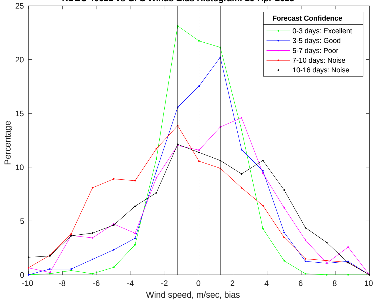
NDBC 46011 vs GFS Winds Bias Histogram: 10-Apr-2025
