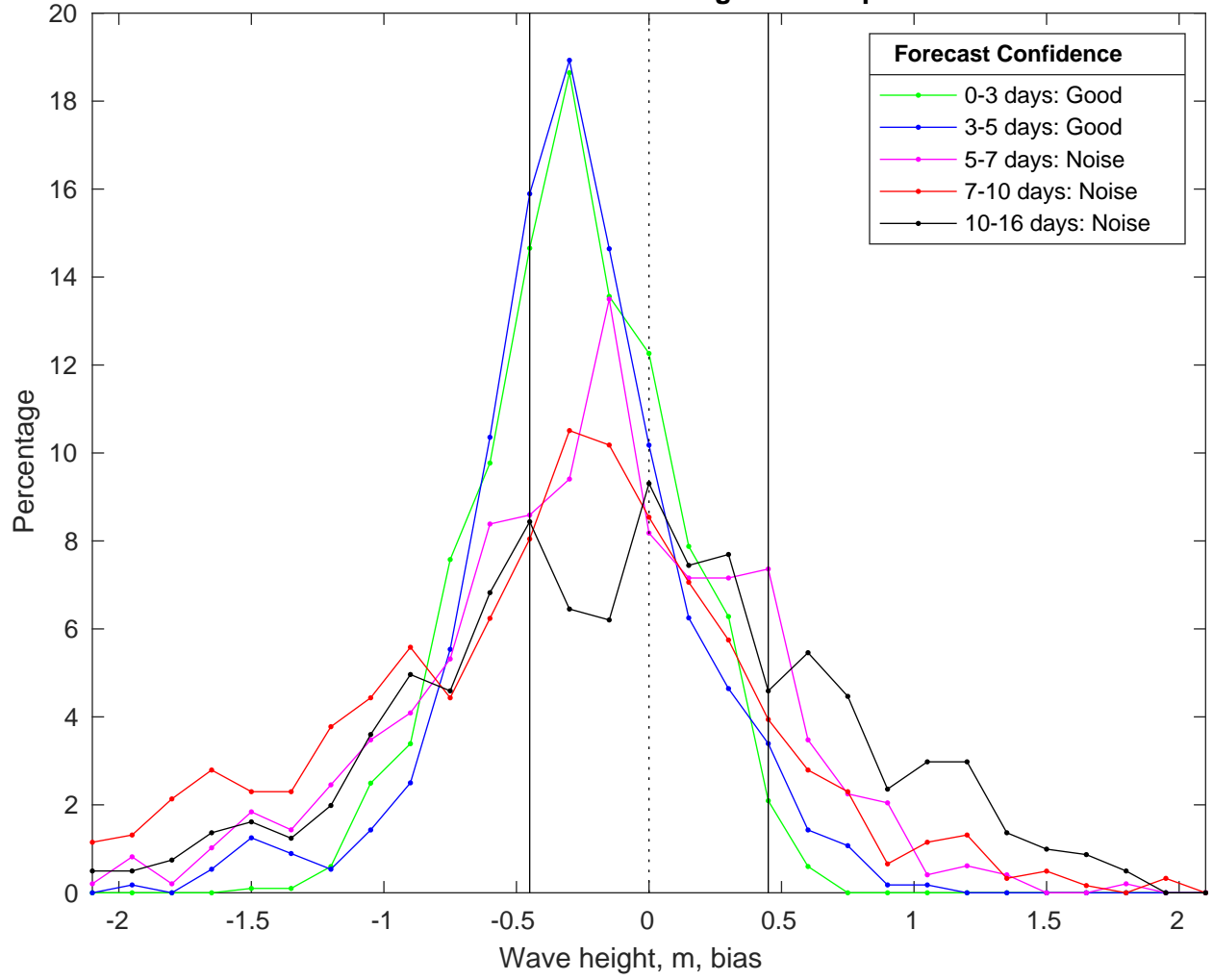
NDBC 46028 vs GFS Waves Bias Histogram: 10-Apr-2025
