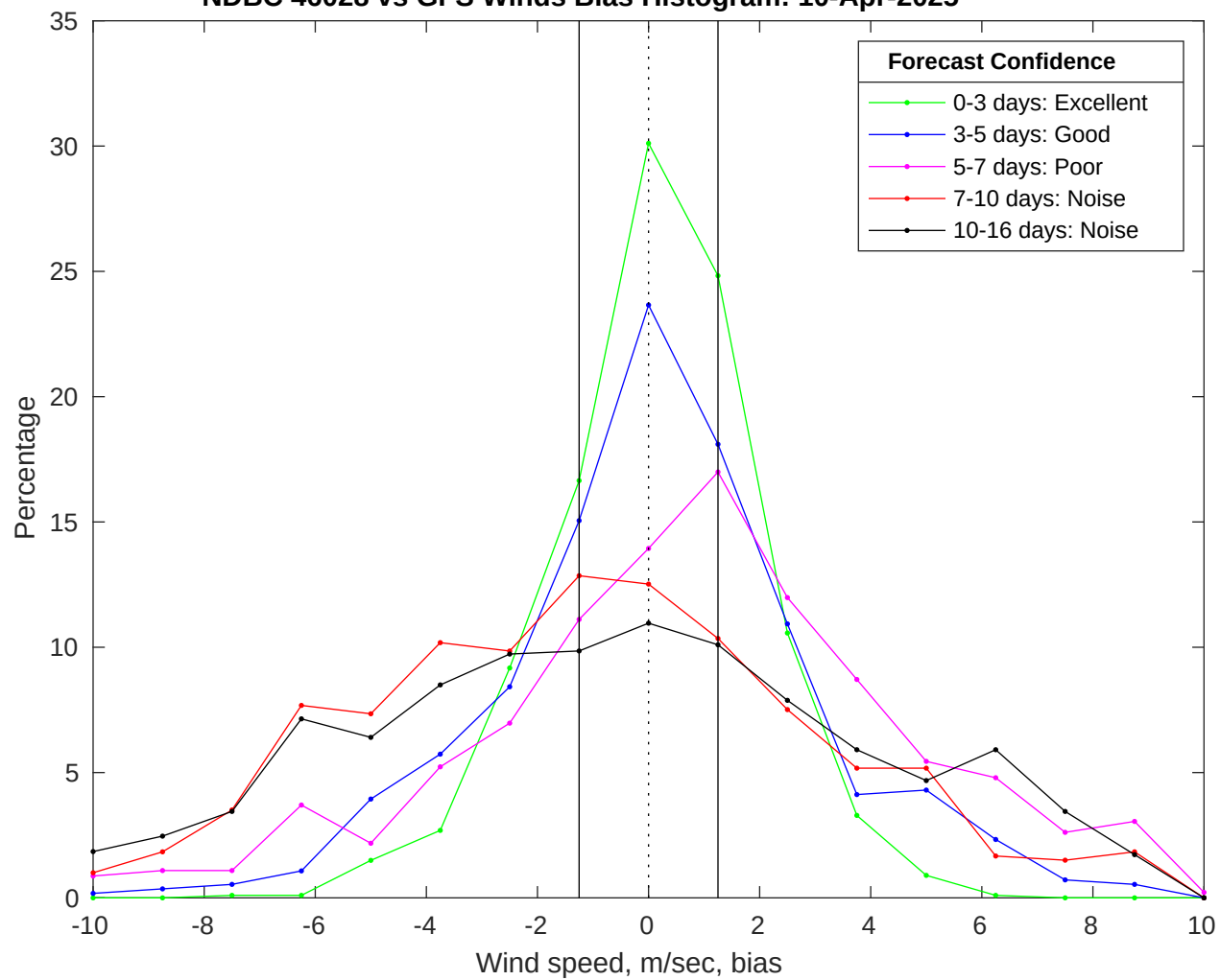
NDBC 46028 vs GFS Winds Bias Histogram: 10-Apr-2025
