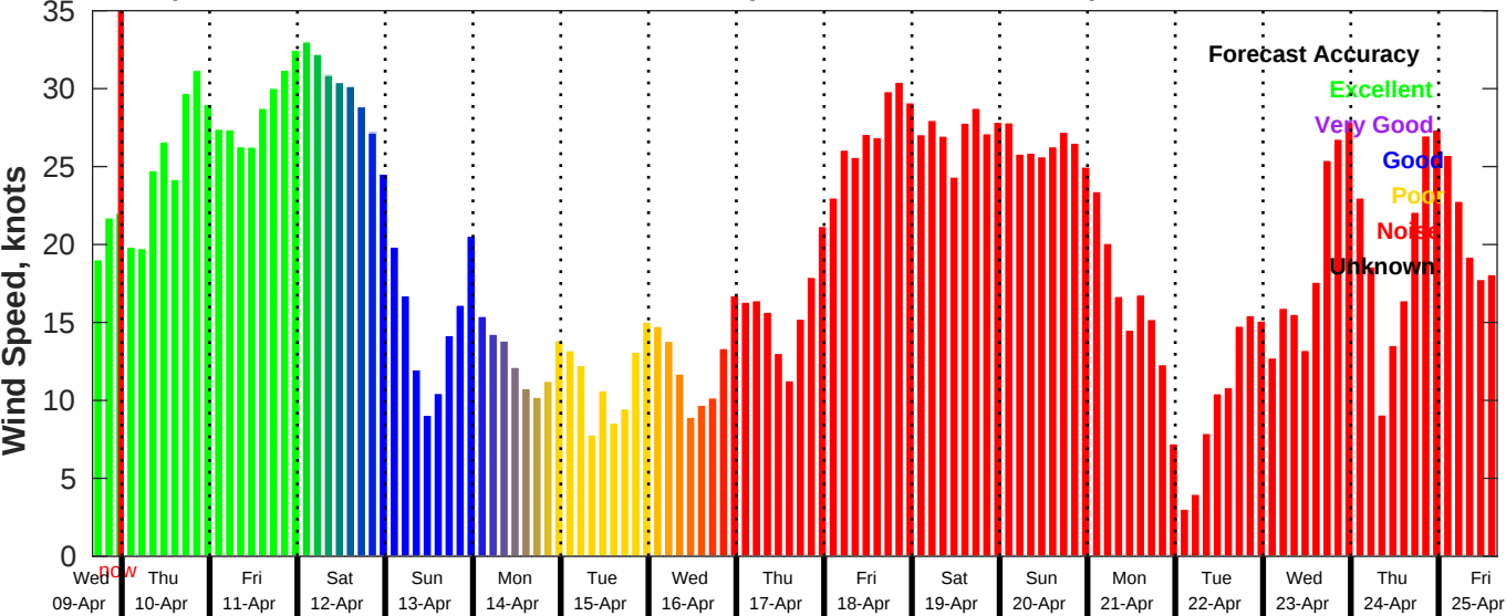
GFS Wind Speed Forecast for NDBC 46028 from 09-Apr-2025 16:00:00 to 25-Apr-2025 16:00:00
