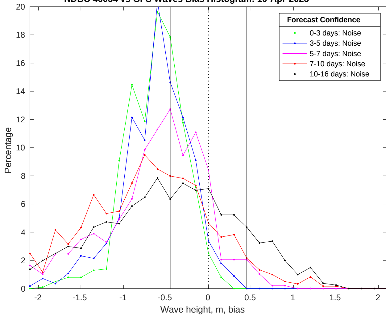
NDBC 46054 vs GFS Waves Bias Histogram: 10-Apr-2025
