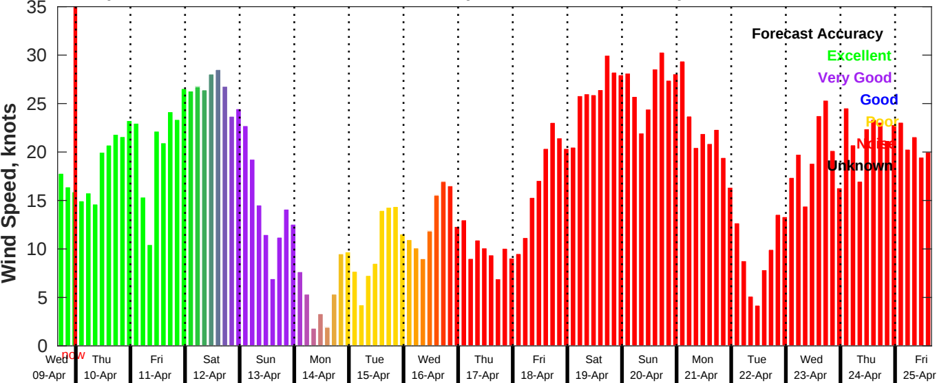
GFS Wind Speed Forecast for NDBC 46054 from 09-Apr-2025 16:00:00 to 25-Apr-2025 16:00:00
