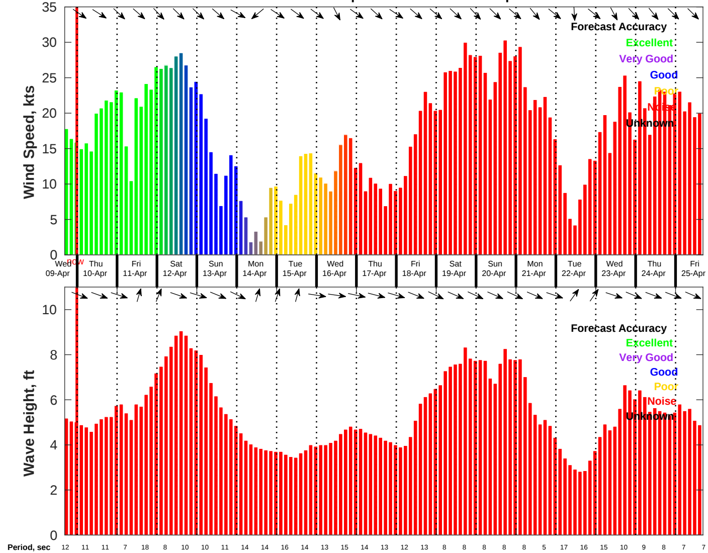
Wind & Wave Forecast for NDBC 46054 from 09-Apr-2025 16:00:00 to 25-Apr-2025 16:00:00
