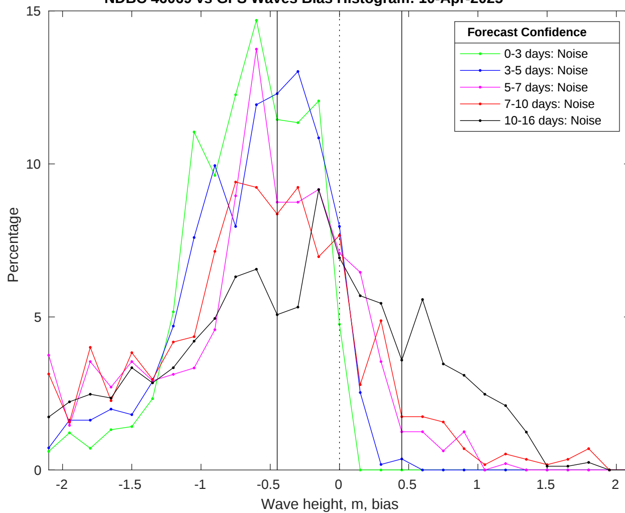
NDBC 46069 vs GFS Waves Bias Histogram: 10-Apr-2025
