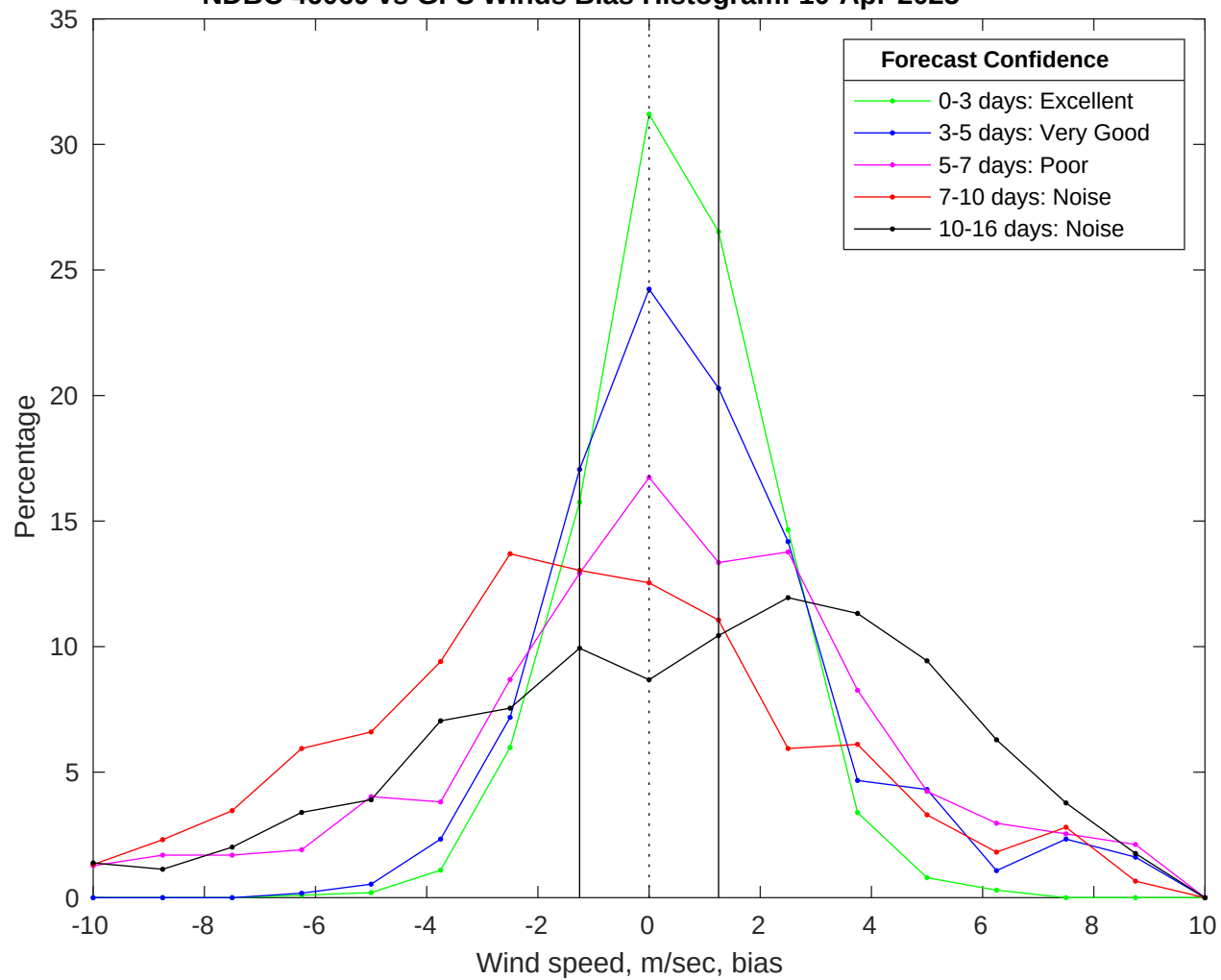
NDBC 46069 vs GFS Winds Bias Histogram: 10-Apr-2025
