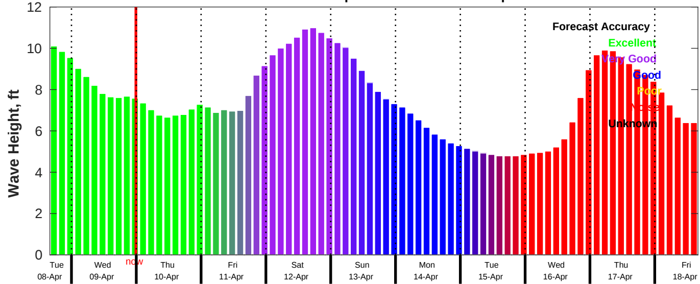
CMEMS Wave Forecast for NDBC 46069 from 08-Apr-2025 16:00:00 to 18-Apr-2025 16:00:00
