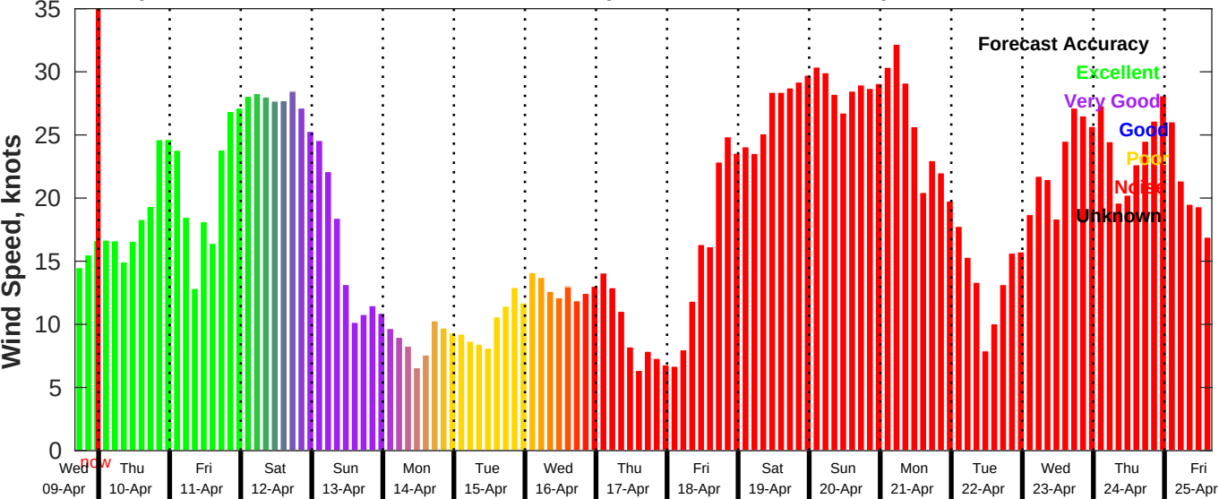
GFS Wind Speed Forecast for NDBC 46069 from 09-Apr-2025 16:00:00 to 25-Apr-2025 16:00:00
