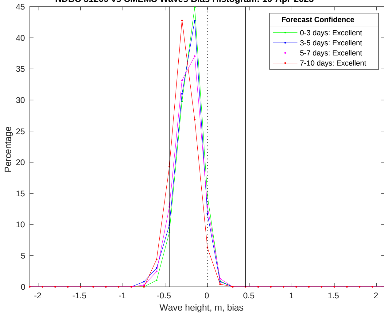
NDBC 51209 vs CMEMS Waves Bias Histogram: 10-Apr-2025
