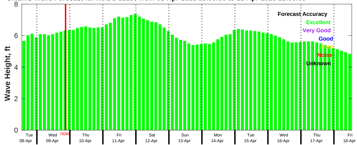
CMEMS Wave Forecast for NDBC 51209 from 08-Apr-2025 13:00:00 to 18-Apr-2025 13:00:00
